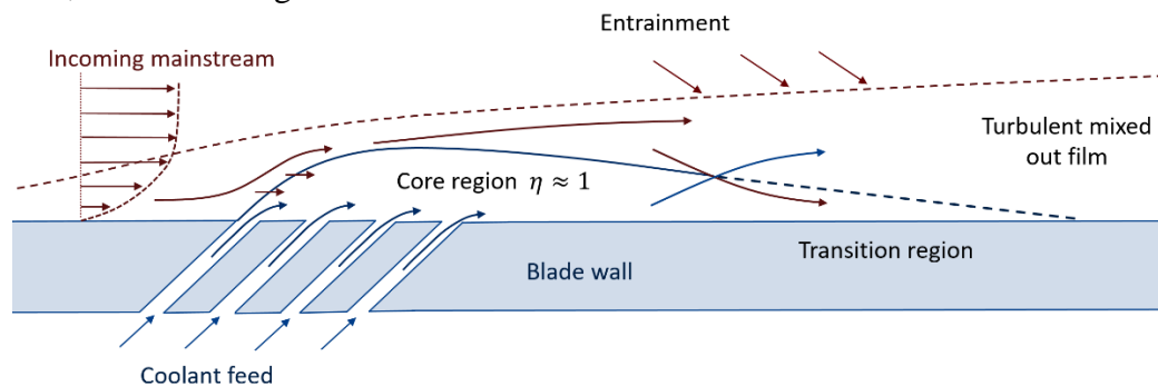
Figure 13 Conceptual model of high porosity films
