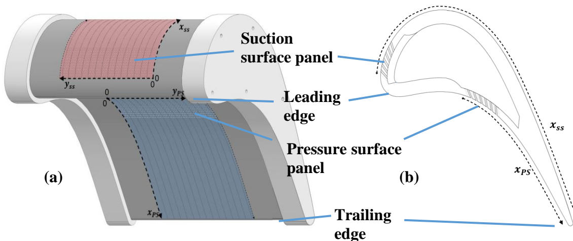
Figure 3 Schematic of geometries and locations used in film effectiveness experiments Overview of film effectiveness data and geometries
